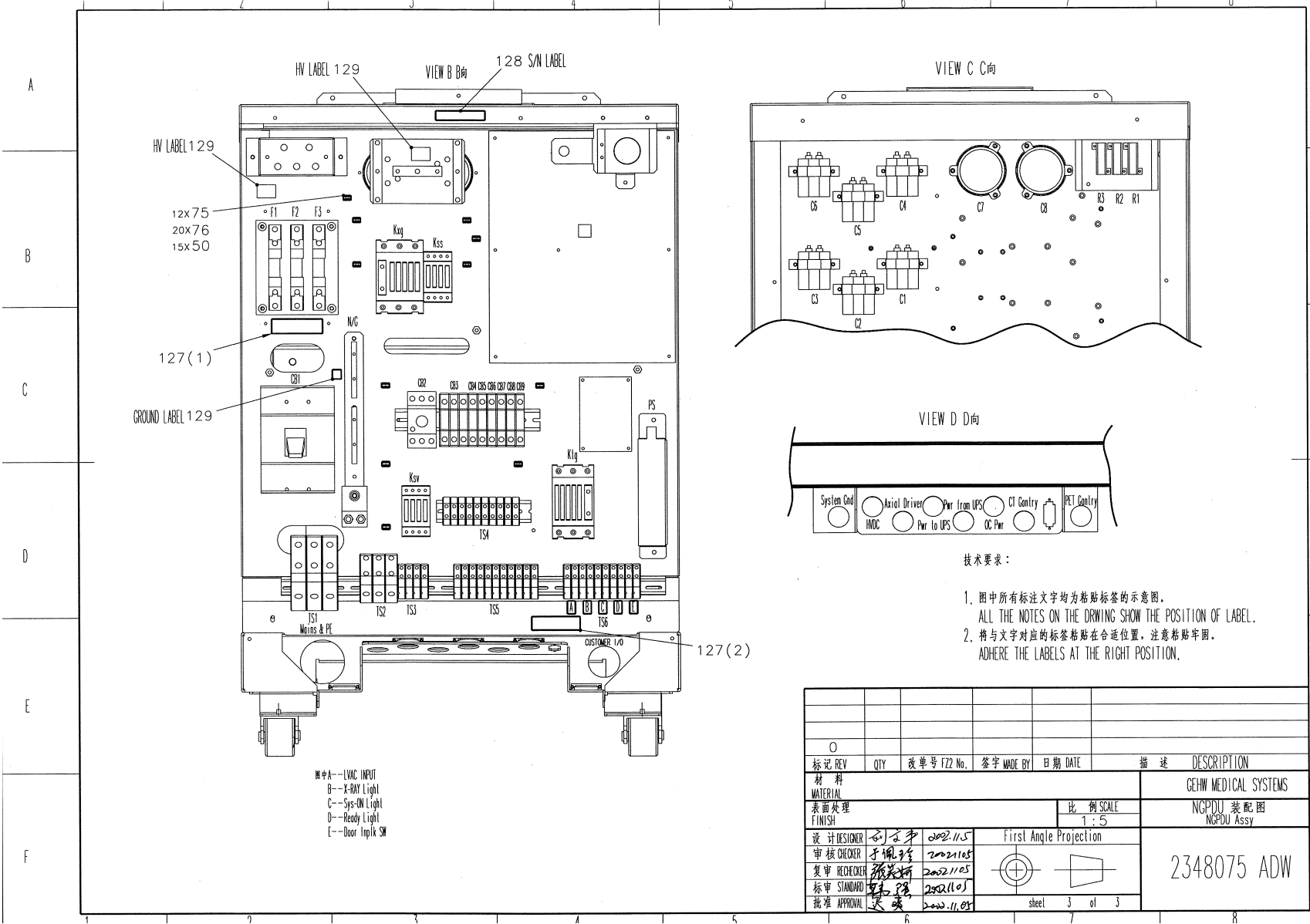
Figure 3-6 NGPDU Assembly2 (2348075, sheet 3, rev 0)
